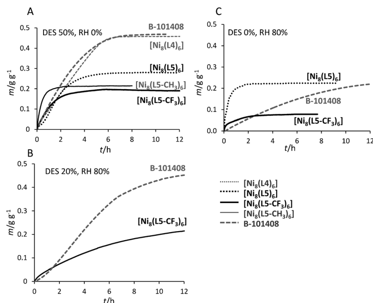
Figure 4. Dynamic adsorption profiles of DES streams for [\text{Ni}_8(\text{L}_4)_6] , [\text{Ni}_8(\text{L}_5)_6] , [\text{Ni}_8(\text{L}_5\text{-CH}_3)_6] , and [\text{Ni}_8(\text{L}_5\text{-CF}_3)_6] , as well as for the Blücher-101408 activated carbon, at 293 K, A) under dry conditions and B) at 80% RH ( m = relative weight increase). Dynamic water adsorption at 293 K and 80% RH (C).
